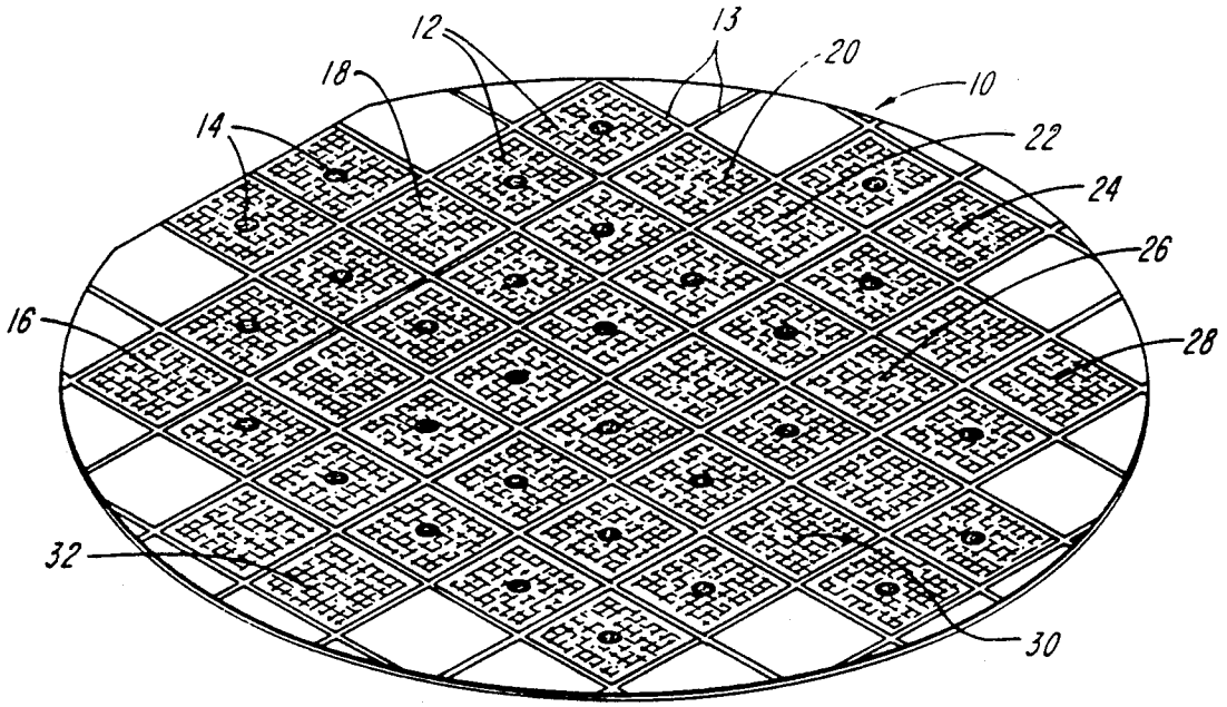
FIG. 1 (PRIOR ART)
